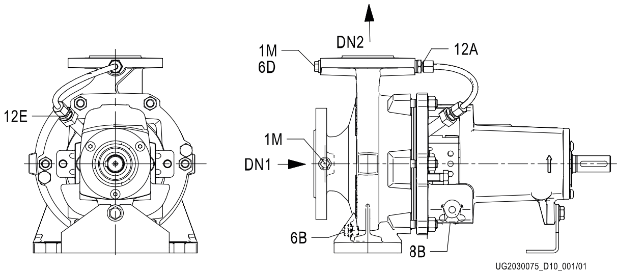
Fig. 5: Version with grease lubrication, no hole for connecting measuring equipment, with connection for pressure gauge
