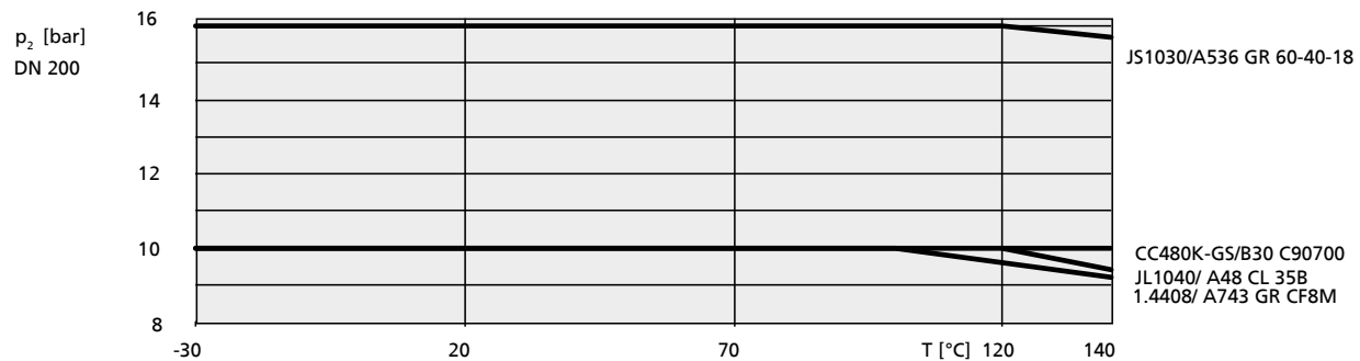
Fig. 2: Pump pressure limits and temperature limits DN 200 for ETN 30)
