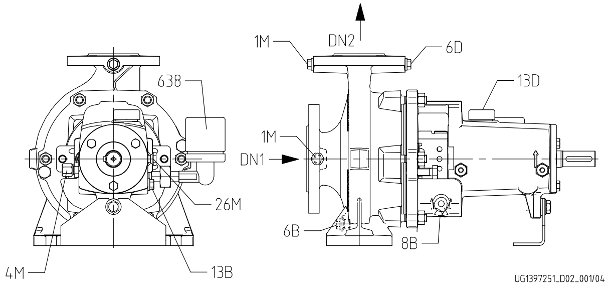
Fig. 4: Version with constant level oiler, with hole for connecting measuring equipment, with connection for pressure gauge
