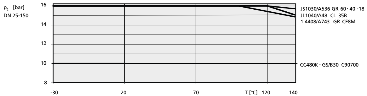
Fig. 1: Pump pressure limits and temperature limits DN 25 - DN 150 for ETN 30)
